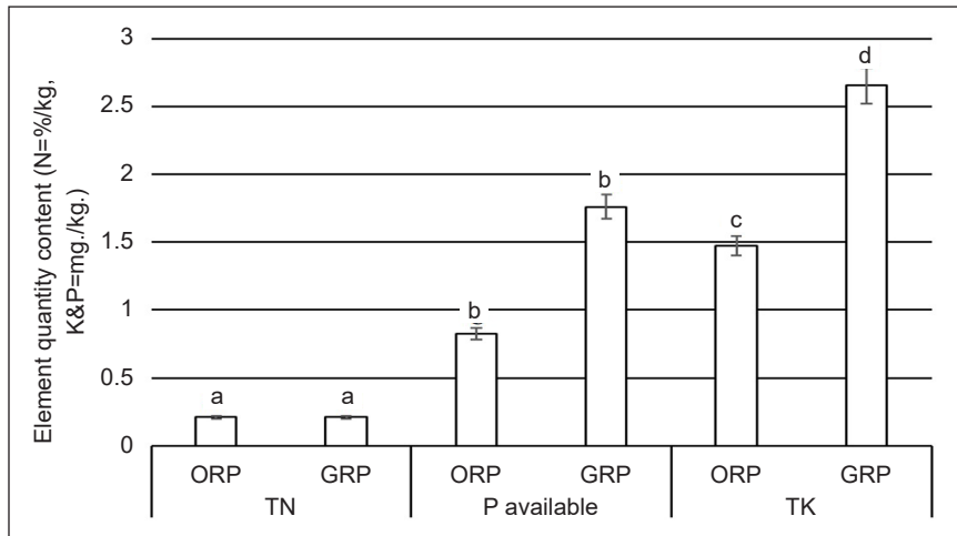
Figure 4. Quantity of macroelements comparison of ORP and GRP in TKR found to TK between ORP and GRP significant ( p < 0.01 )
